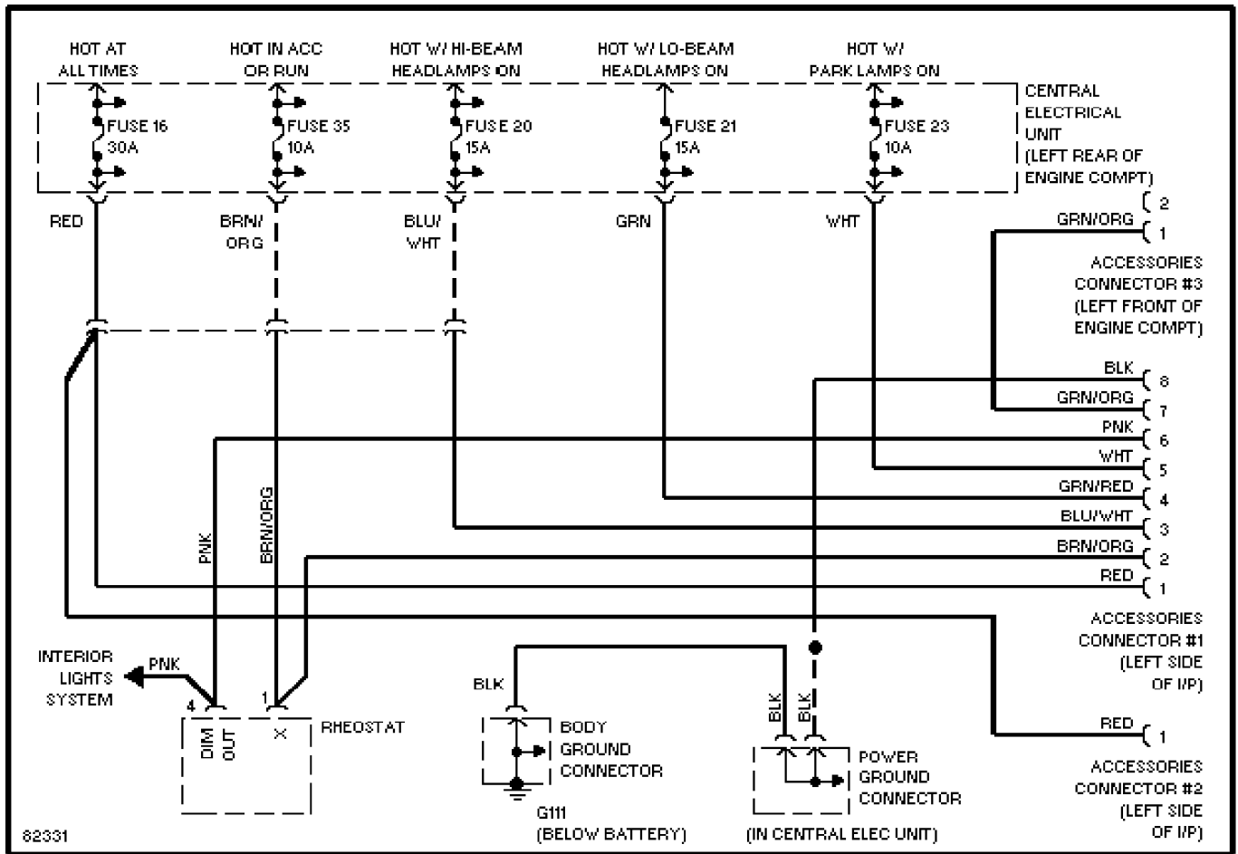
Accessories Connector Circuit, Early Production
