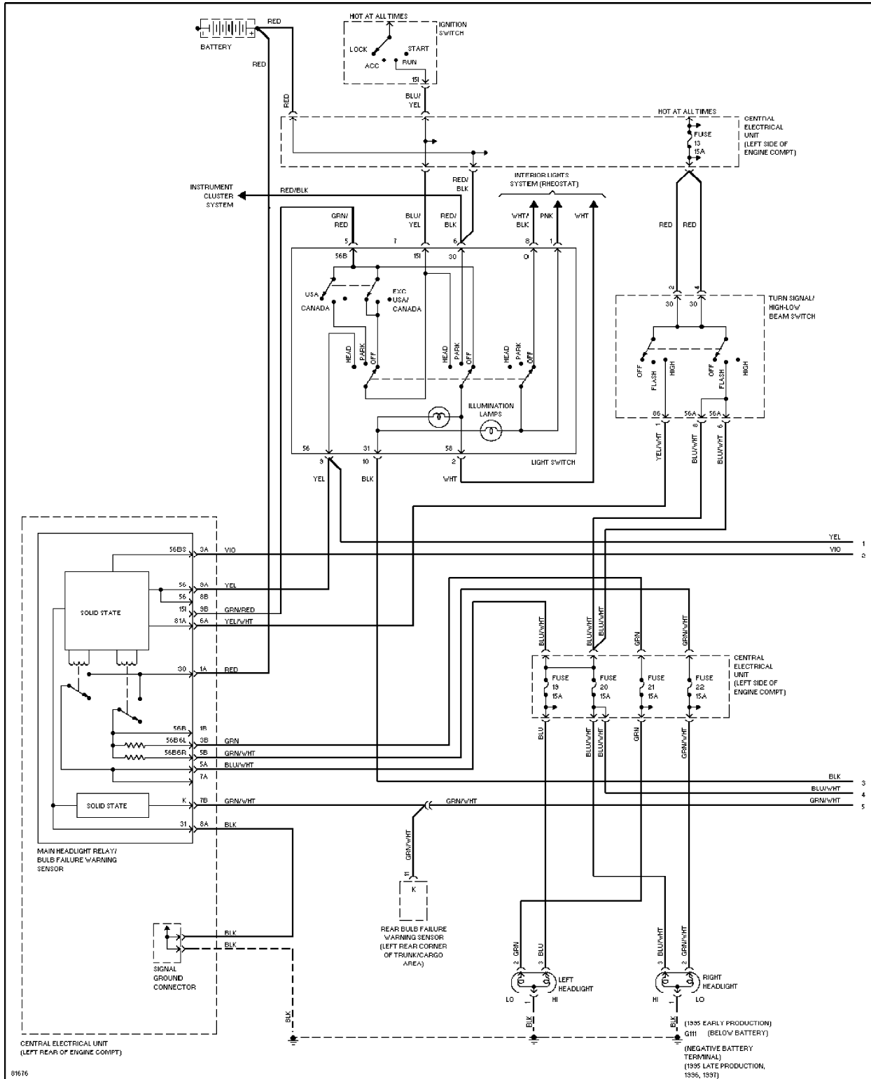
81676 Headlight Circuit (1 of 2)
