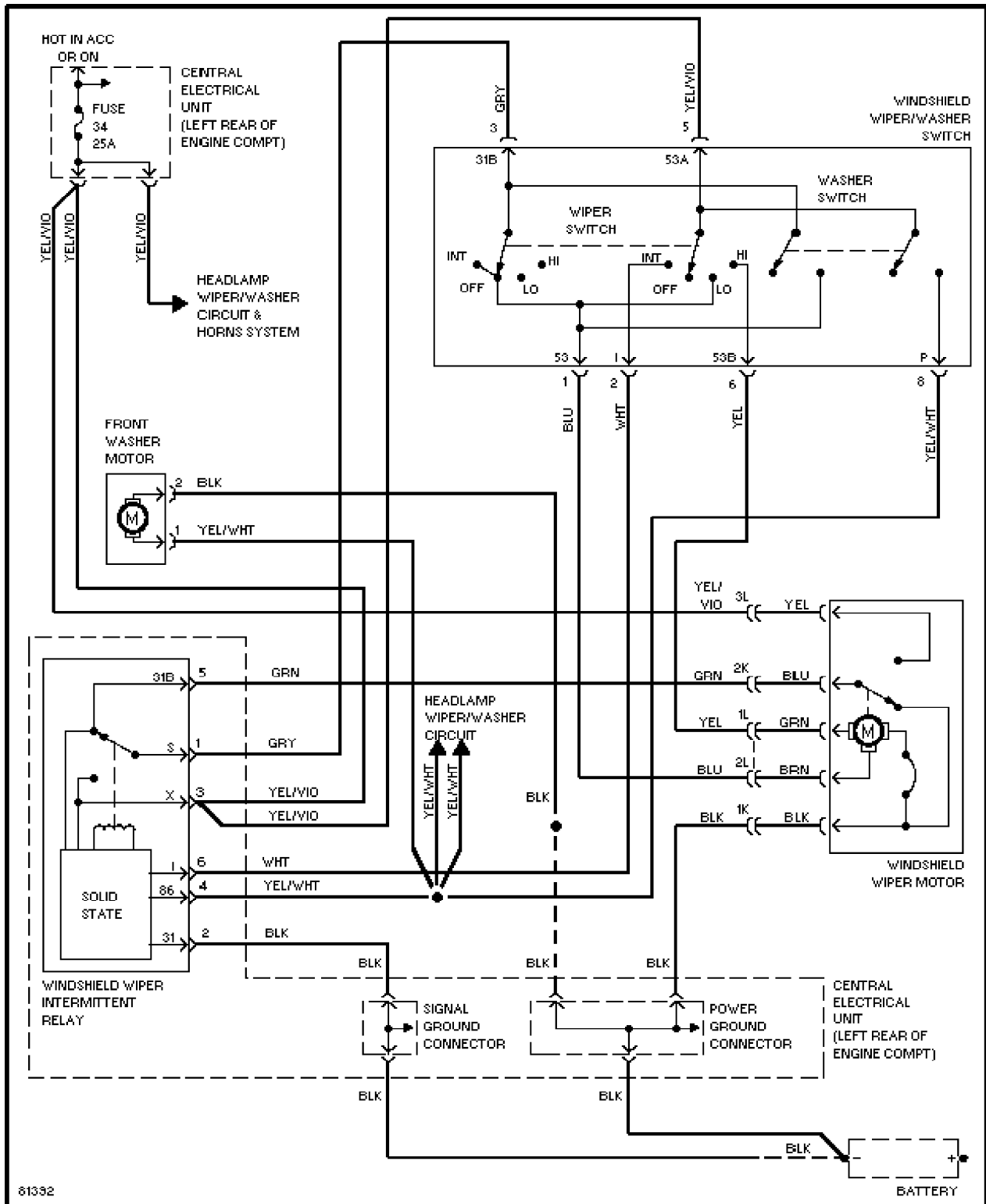
Front Wiper/Washer Circuit, Late Production
