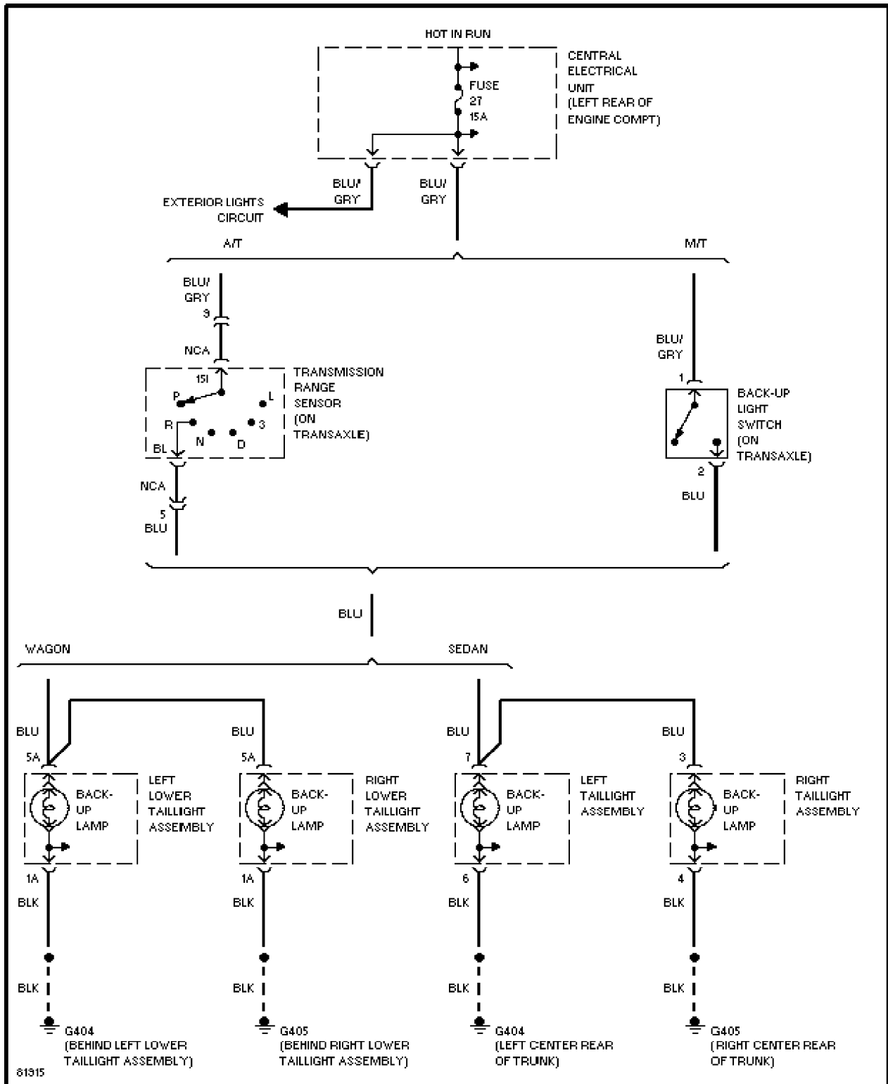
Backup Lamps Circuit, Sedan & Wagon
