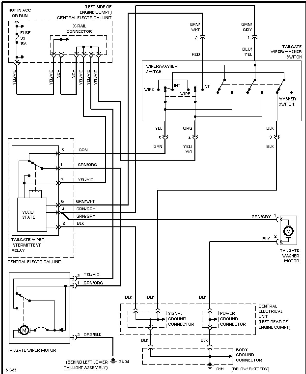
Rear Wiper/Washer Circuit, Early Production
