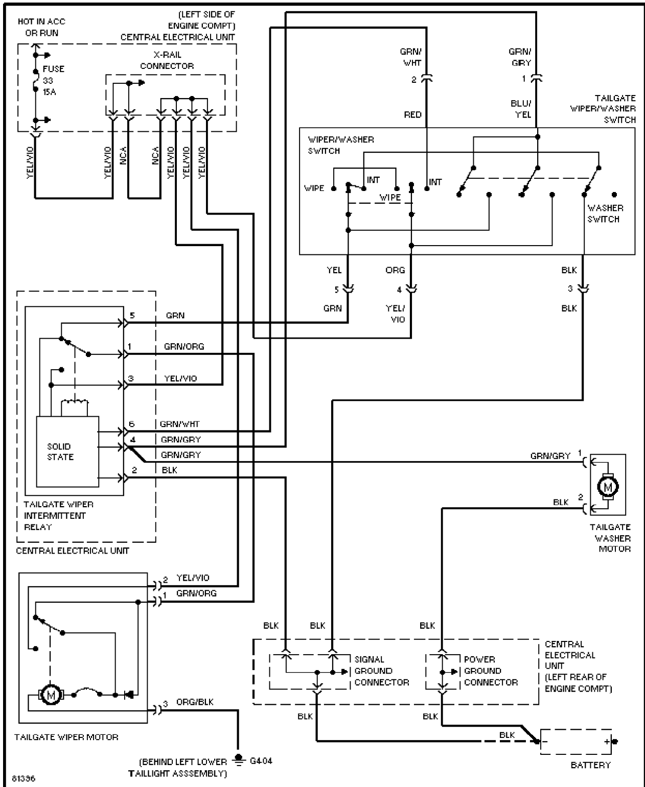
Rear Wiper/Washer Circuit, Late Production
