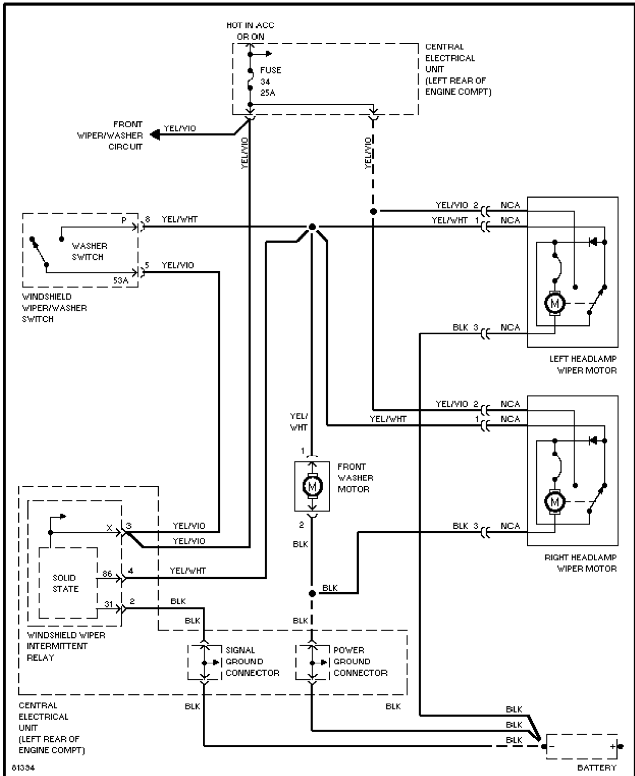
Headlamp Wiper/Washer Circuit, Late Production
