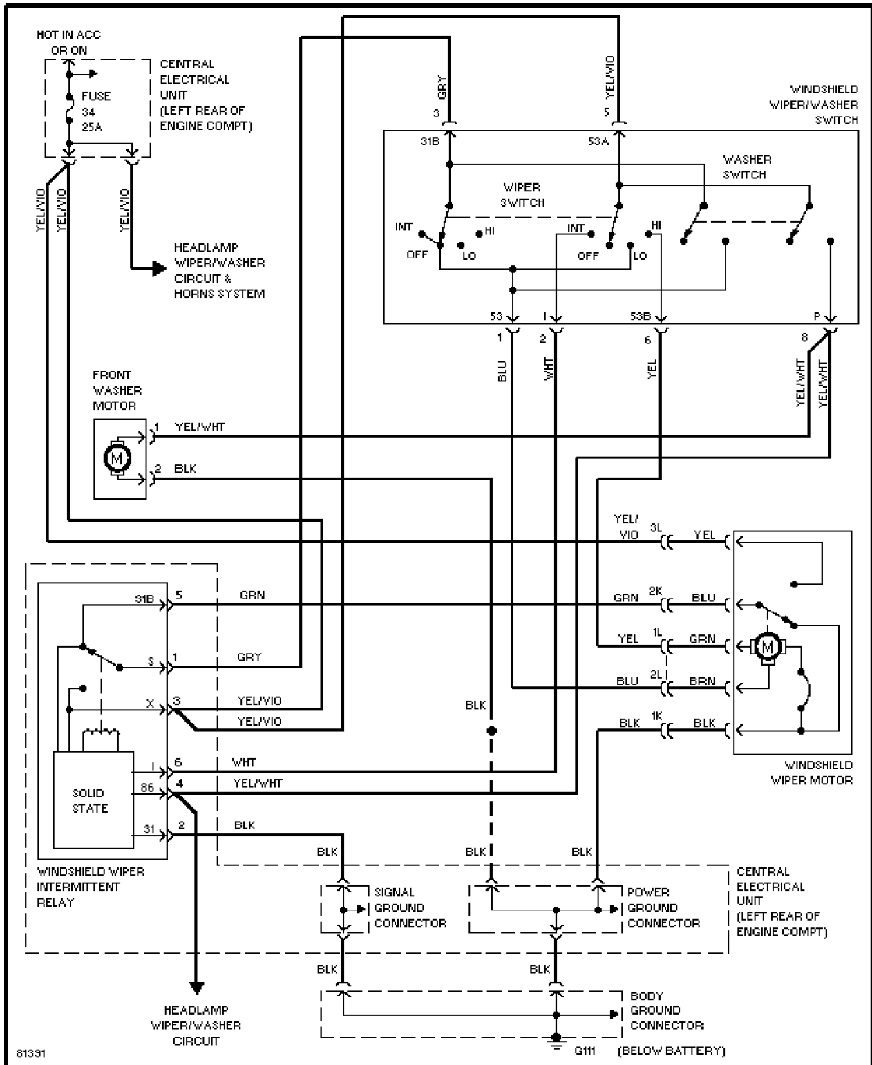
Front Wiper/Washer Circuit, Early Production
